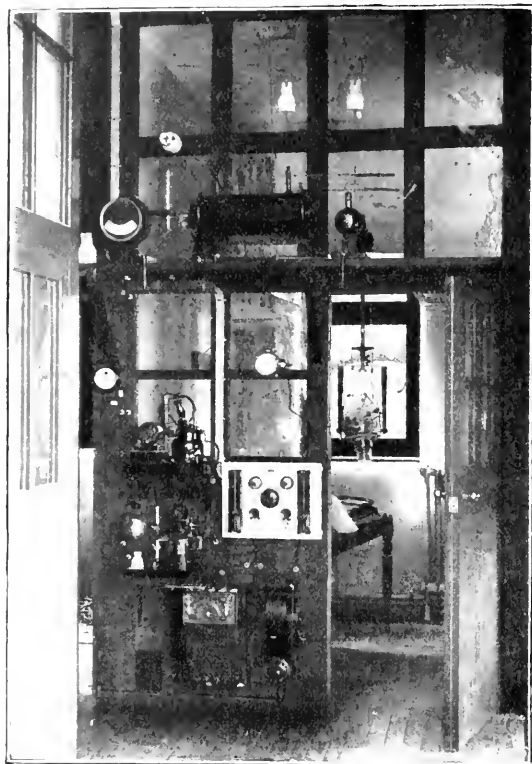
FIG. 185.—X-ray treatment cubicle. ( Archives of Röntgen Ray. ) Control apparatus arranged outside the cubicle.
